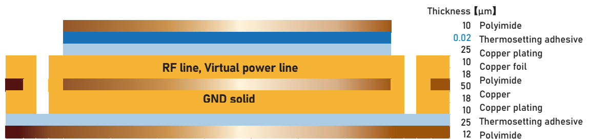
Sample FPC evaluating crosstalk
